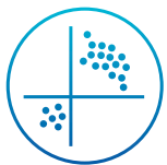
Flow cytometry
